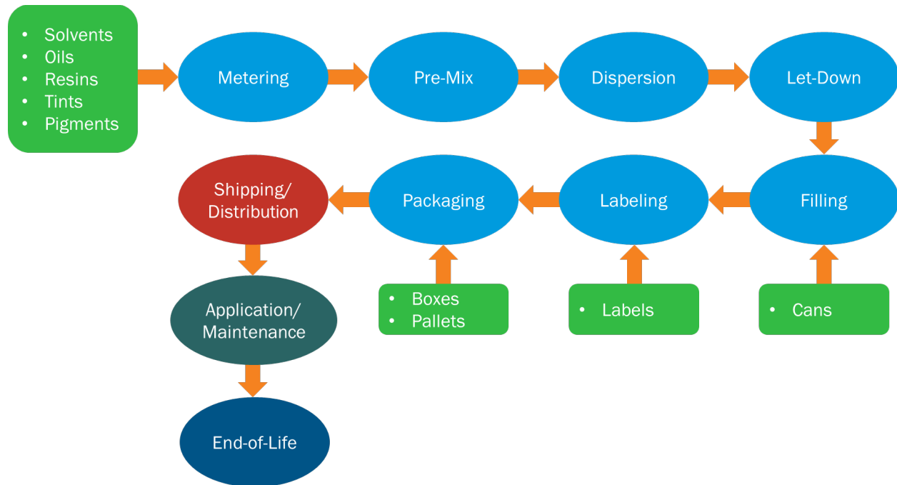
Figure 1. Flow diagram for cradle-to-grave LCA of KILZ 2® All-Purpose Primer
