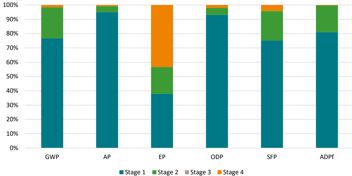
Figure 4. LCIA contribution results for 2000
