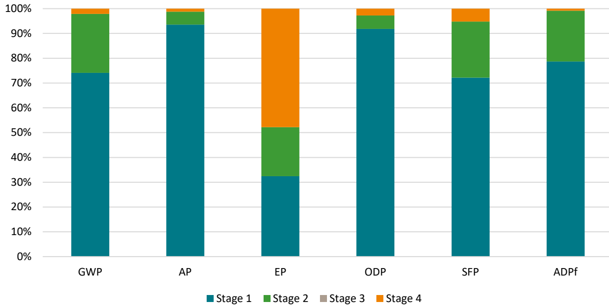
Figure 4. LCIA contribution results for PR040
