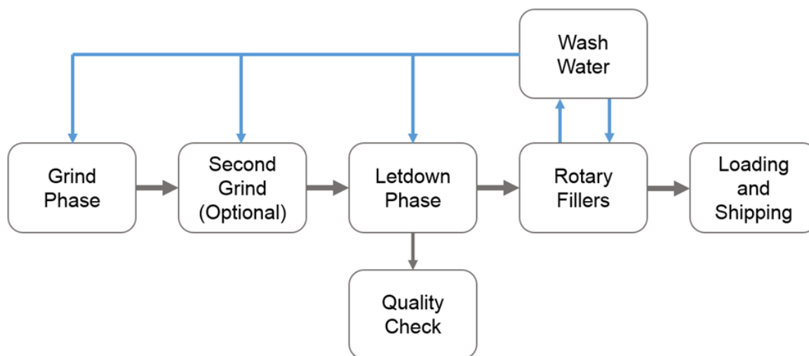
Figure 2: Behr and Masterchem process flow schematic
